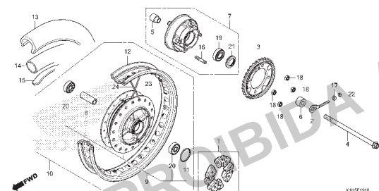
C-19.10 Roda Traseira (BIZ 125 ES)
