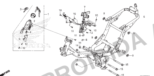
C-39 Chassi
