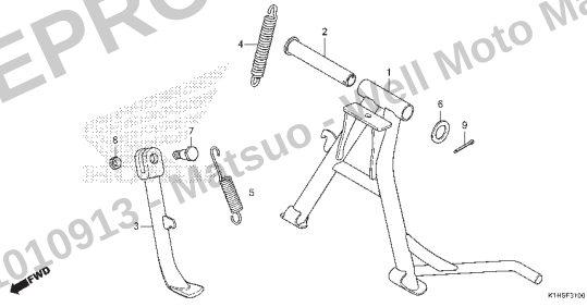
C-31 Cavalete
